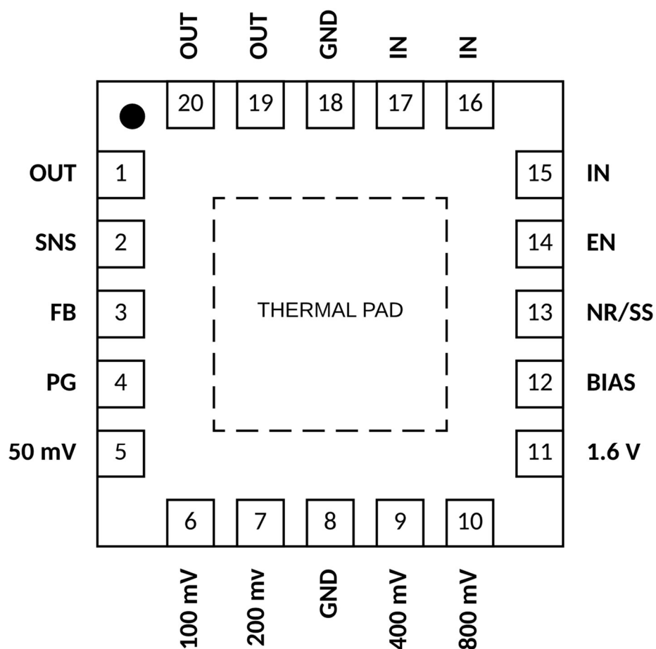
Figure 2 Au8014A Pin Configuration
