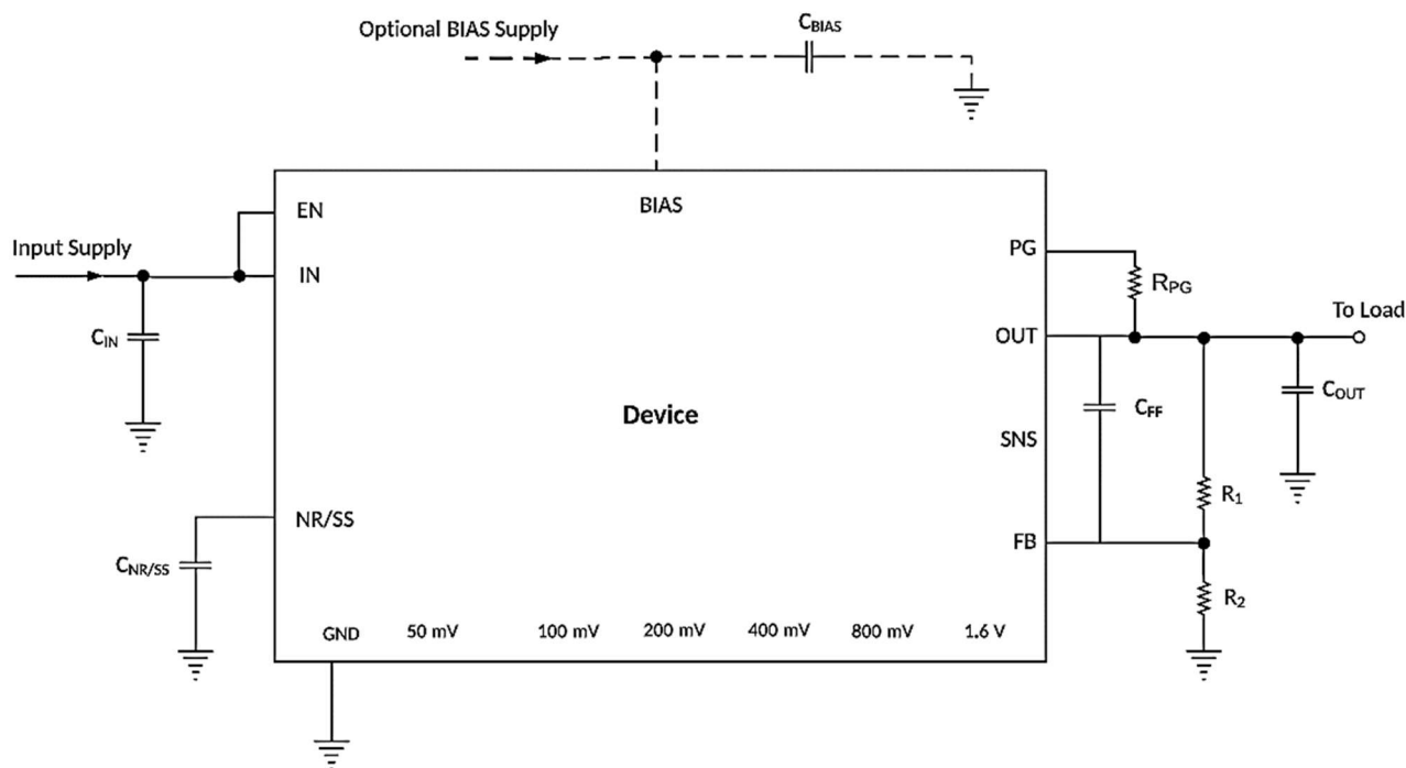
Figure 10 Adjustable Operation
