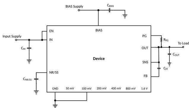
Figure 1 Application Schematic
