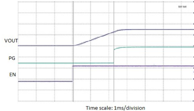
Figure 6 Power On from EN
