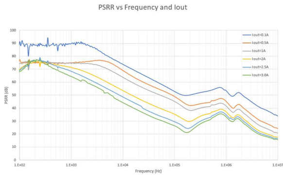
Figure 3 PSRR vs Frequency and I_{OUT}
