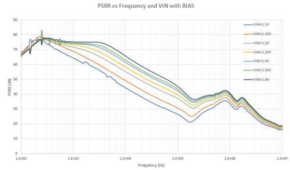
Figure 4 PSRR vs Frequency and V_{IN} with Bias
