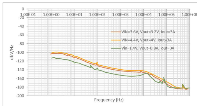
Figure 8 Noise PSD vs Frequency (CNRSS=10nF)
