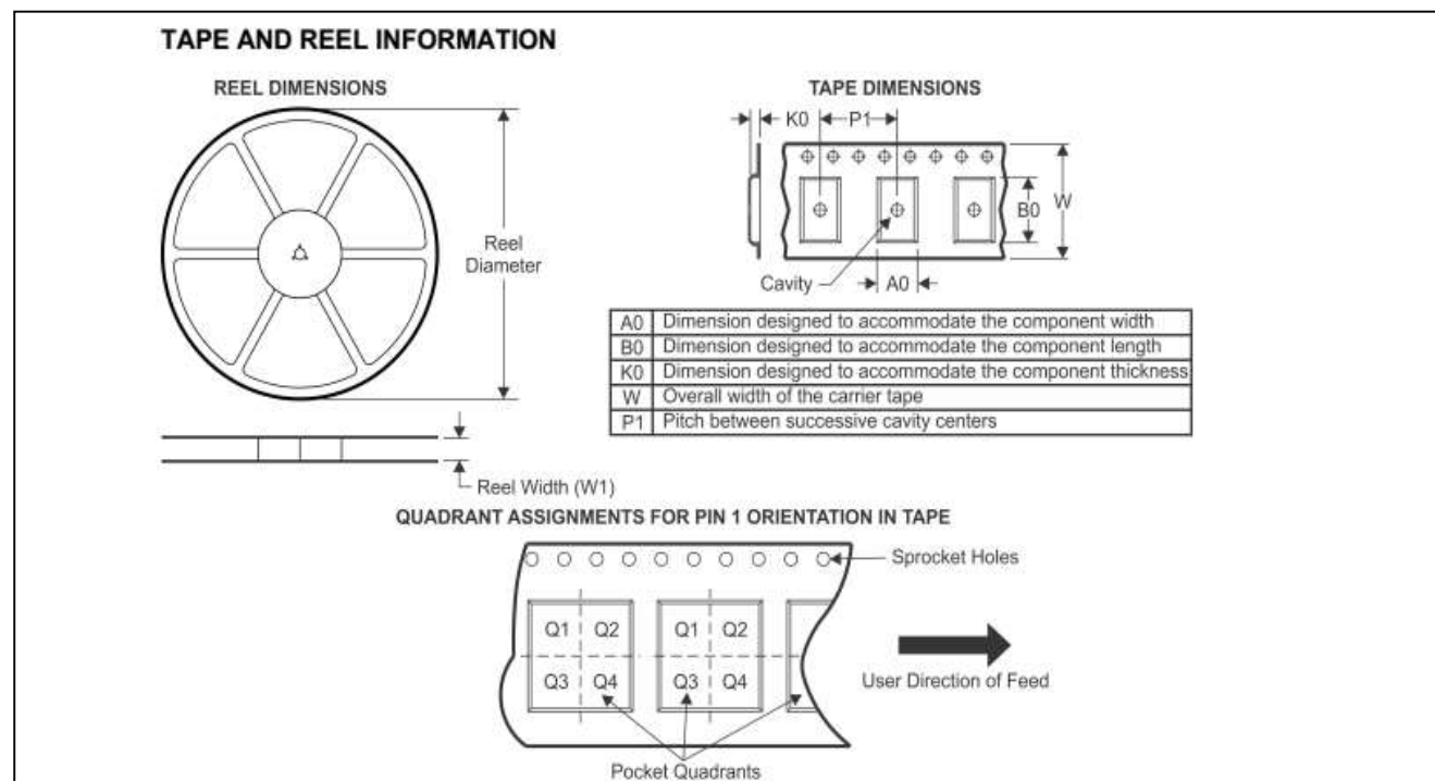
Figure 14 Tape and Reel Drawing
