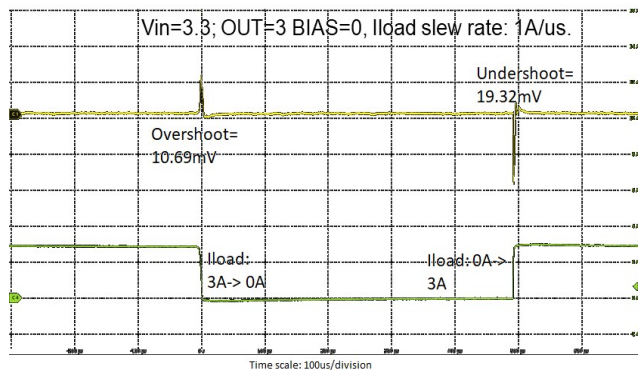
Figure 7 Load Transients
