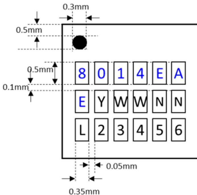
Figure 15 Marking Drawing
