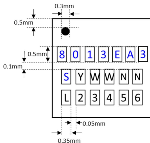
Figure 15 Marking Drawing
