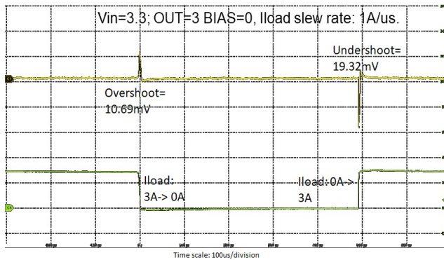
Figure 7 Load Transients
