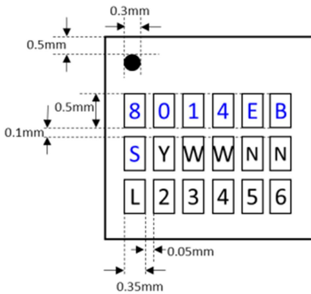
Figure 15 Marking Drawing
